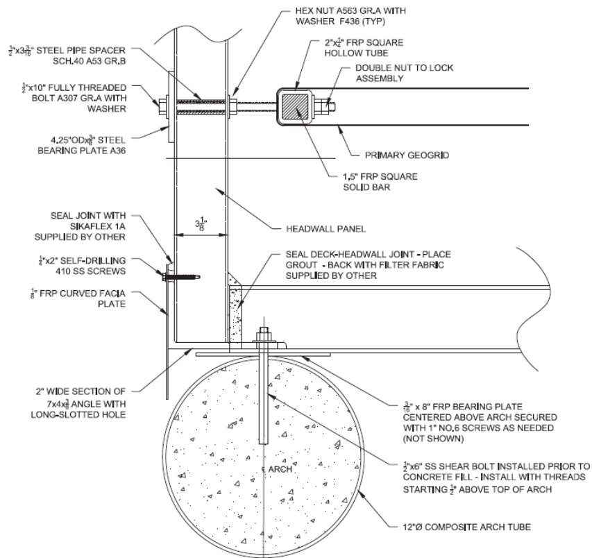
Figure 11 Cross section of the MSE headwalls connection to the arch system (ATI)
