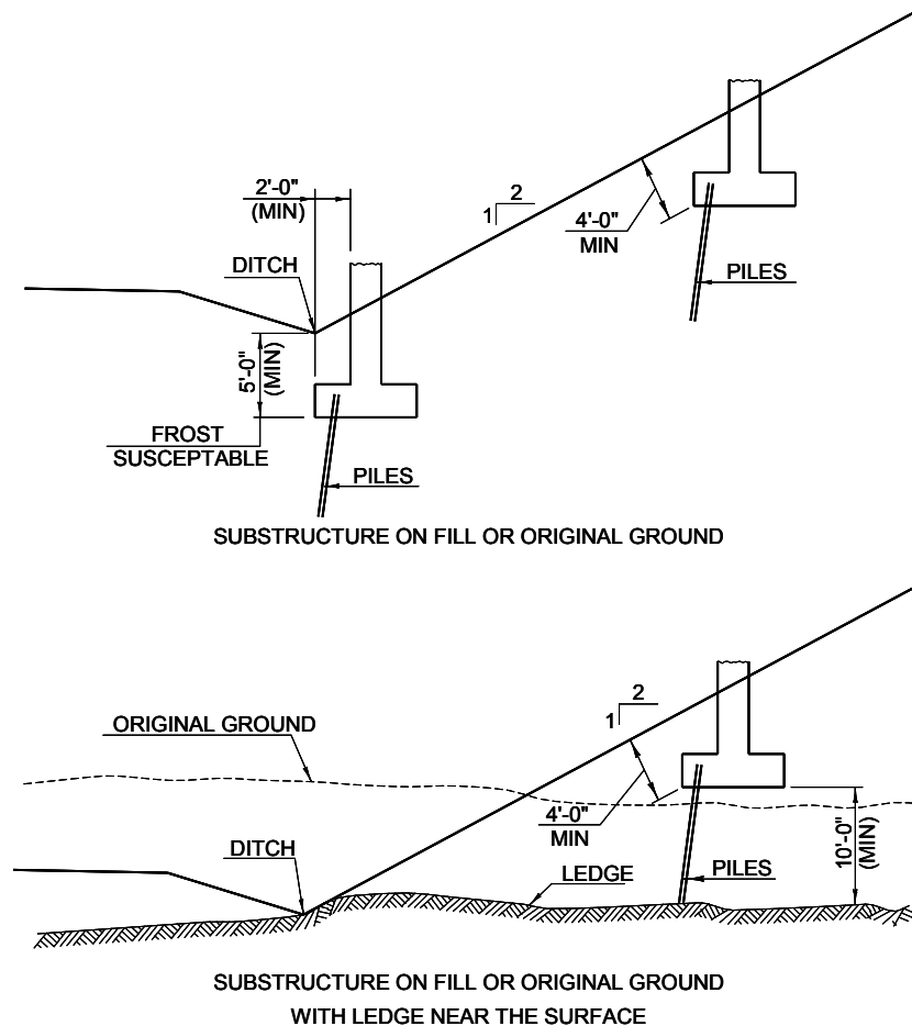
Figure 11.3.1-1 Substructures - Foundation Treatment
