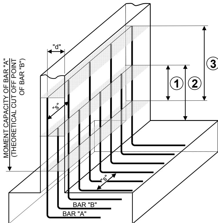
Figure 5.5.5 -1 Cat. 1: Alternate Bars Terminated
