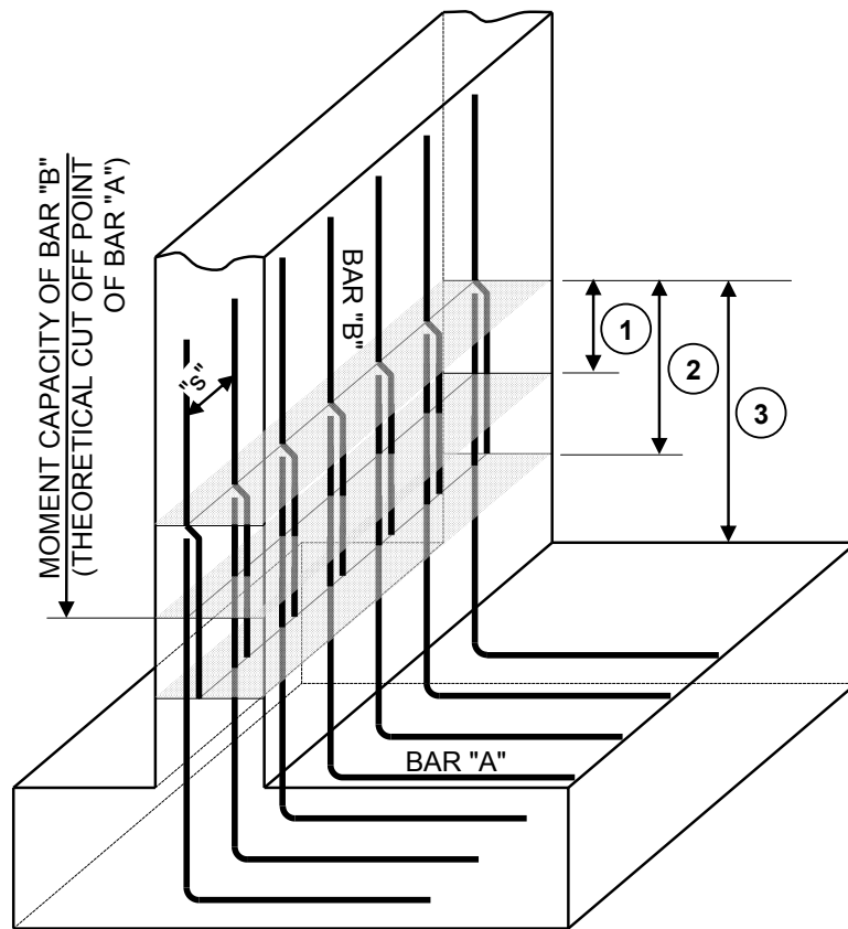
Figure 5.5.5 -3 Cat. 3: Bars Spliced above the Footing
