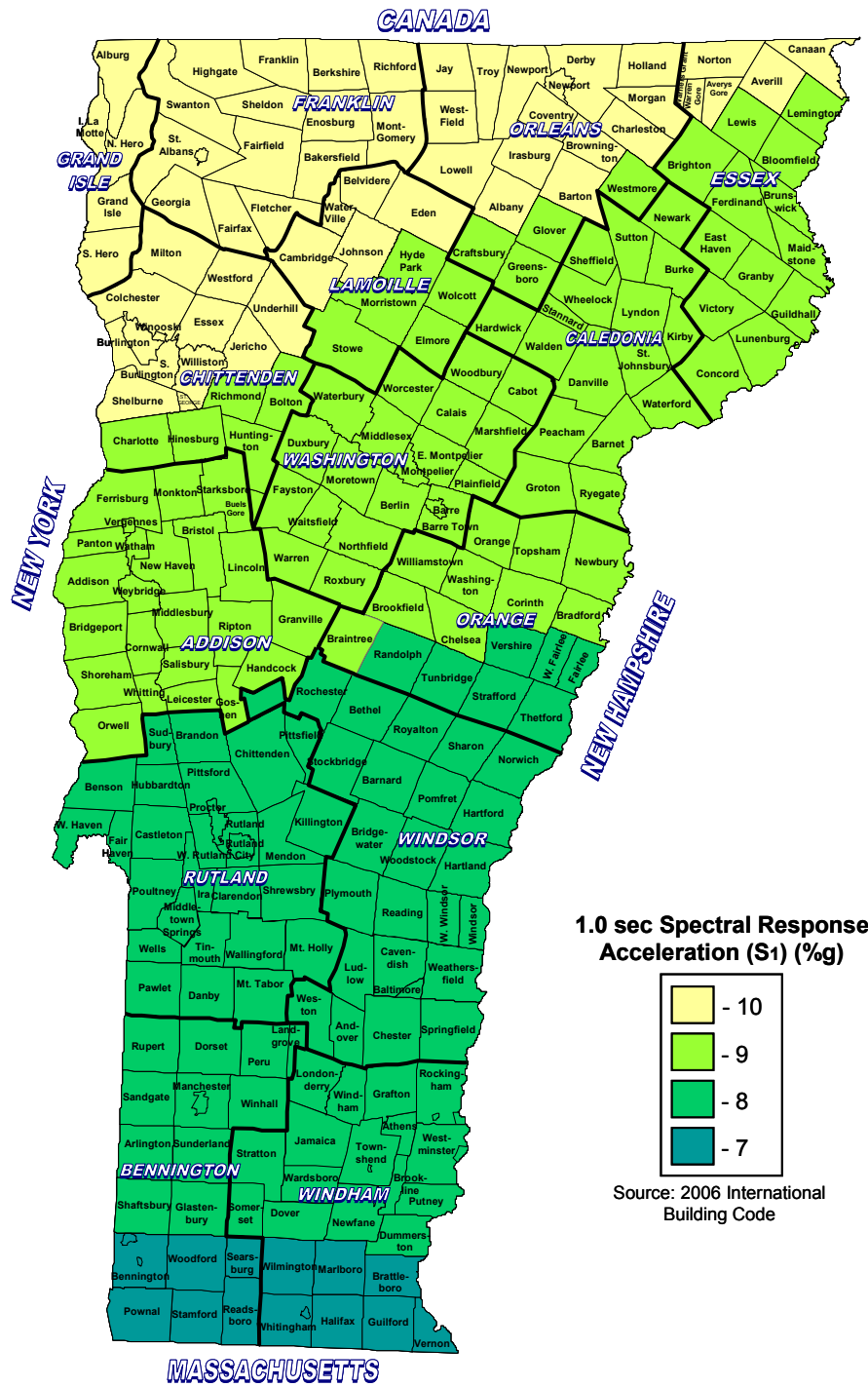
Figure 3.8.3 -1 Maximum Considered Earthquake ground motion for Vermont of 1.0 sec. Spectral Response Acceleration (S 1 ) (5 percent of critical damping), Site Class B (2006 International Building Code)
