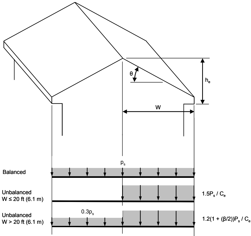
Figure 3.7.2.2.2 -1 Balanced and Unbalanced Snow Loads for Hip and Gable Roofs (ASCE 7-05 Figure 7-5)
