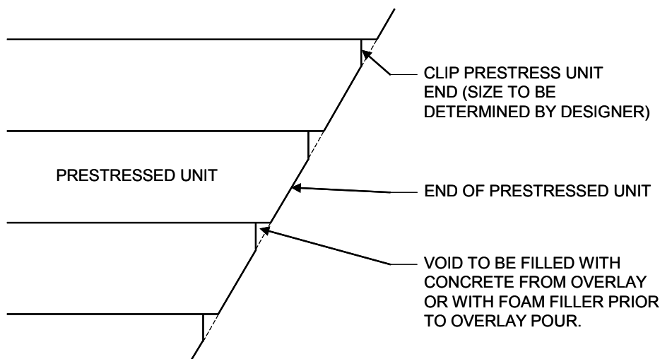
Figure 5.3.1 -1 Clip detail for skews greater than 30°
