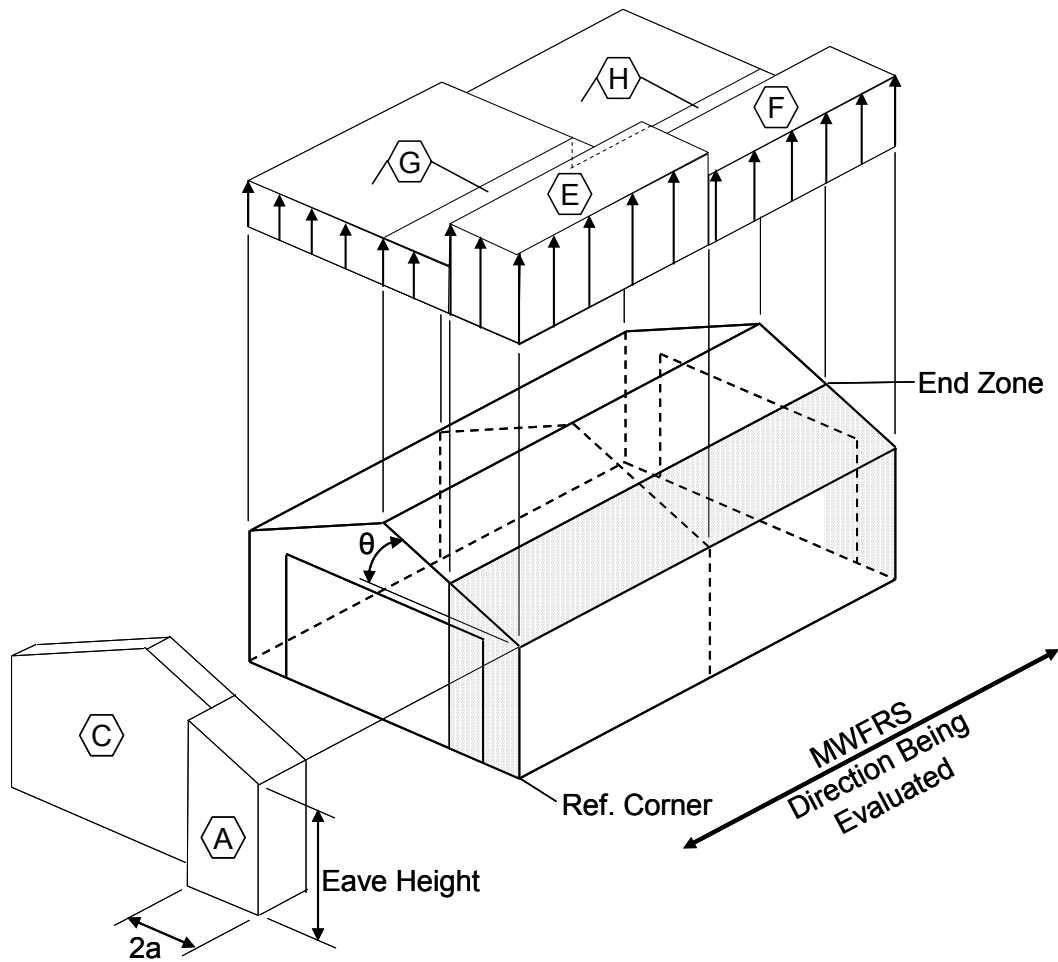
Figure 3.6.3.6.1 -2 Main Wind Force Resisting System (MWFRS) in Transverse Direction (Source: ASCE 7-05 Figure 6-2)
