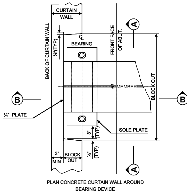
Figure 14.3.1.1.2 -1 Plan detail of Curtain Wall Bearing Box Out
