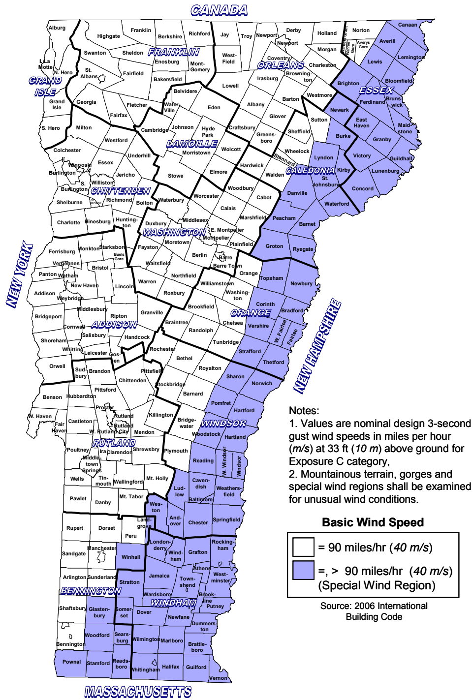
Figure 3.6.3 -1 Vermont Basic Wind Speed (3-Second Gust) (2006 International Building Code)
