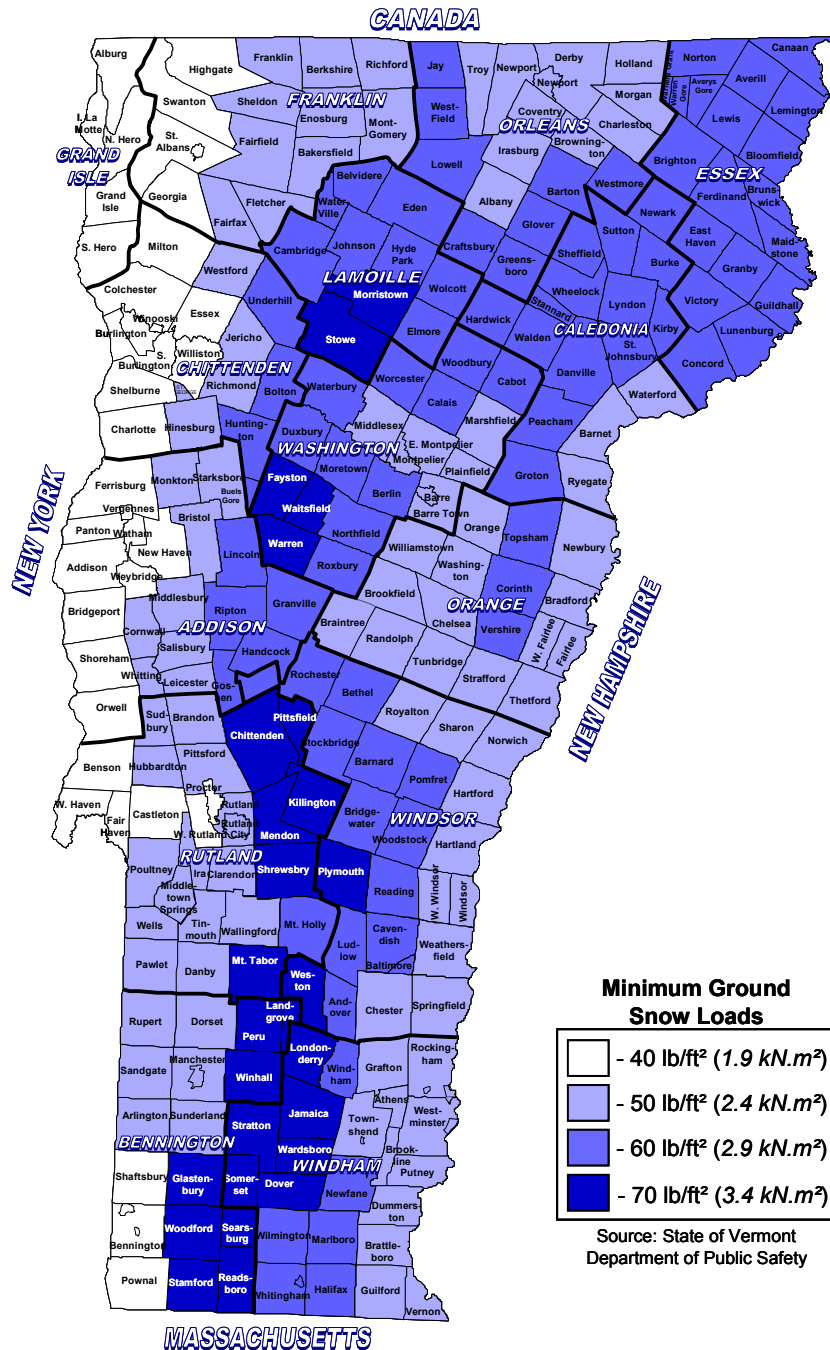
Figure 3.7.2 -1 Minimum Ground Snow Loads (The Vermont Department of Public Safety)
