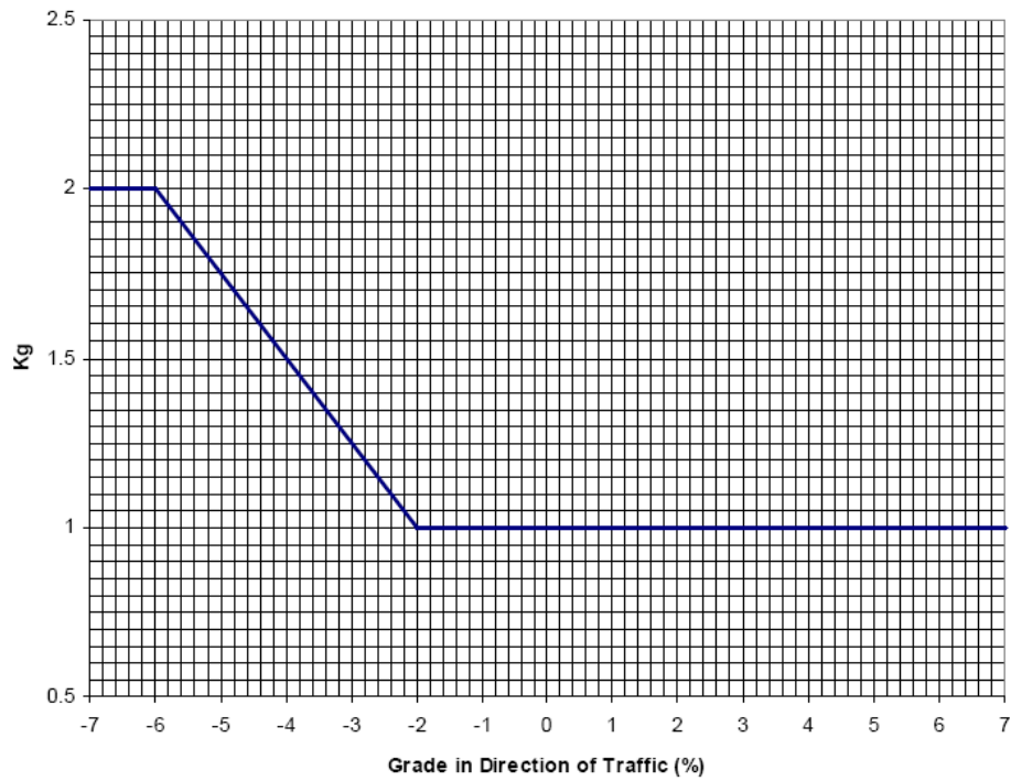
Figure 13.4 -1 Grade Traffic Adjustment Factor (Kg)
