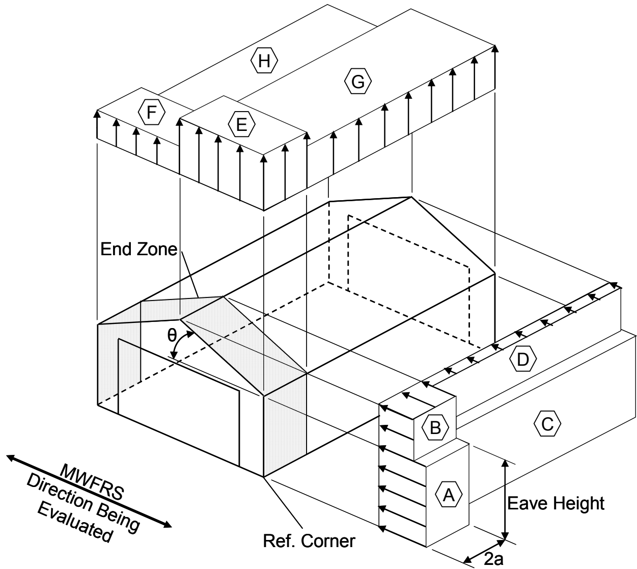
Figure 3.6.3.6.1 -3 Main Wind Force Resisting System (MWFRS) in Longitudinal Direction (Source: ASCE 7-05 Figure 6-2)
