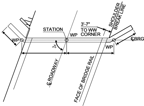
Figure 2.3.1-1 Deck on Beam Bridge Layout
