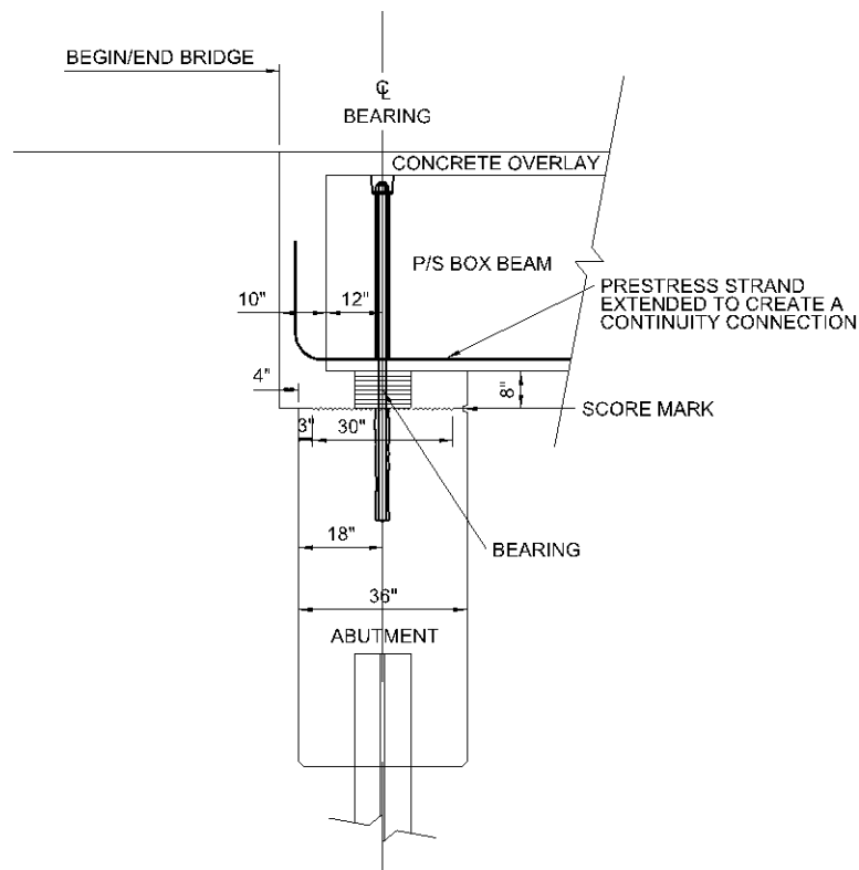
Figure 5.7.2 -1 Box Beam Type B Bridge End Detail
