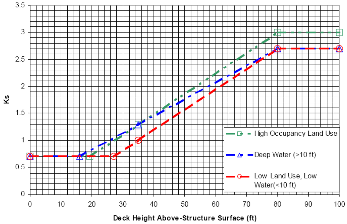
Figure 13.4 -3 Traffic Adjustment Factor (Ks) for Deck Height and Under Conditions
