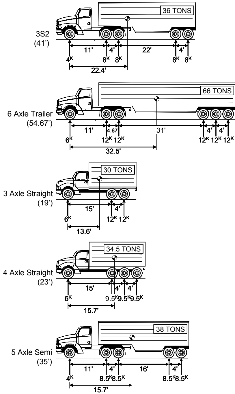
Figure 15.2-1 Vermont Standard Load Rating Trucks
