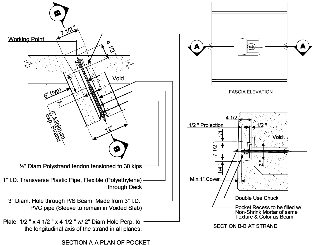
Figure 5.3.6.1 -2 Transverse Post-Tensioning Pocket *AASHTO M270 Grade 50 steel (M270/M270M, Grade 345 Steel)
