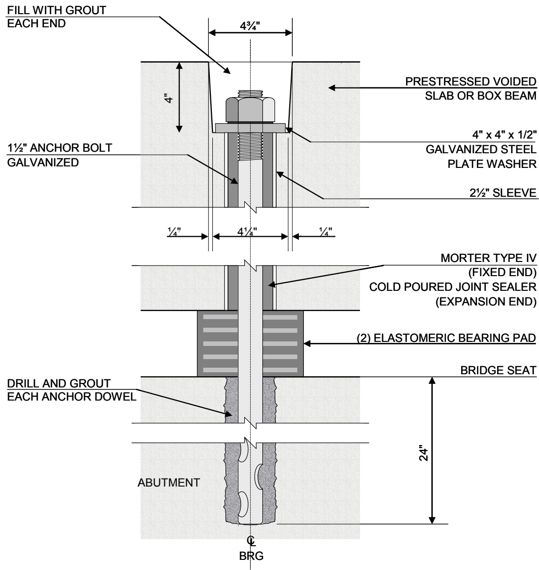
Figure 5.4.1 -1 Prestress Beam Anchor Detail
