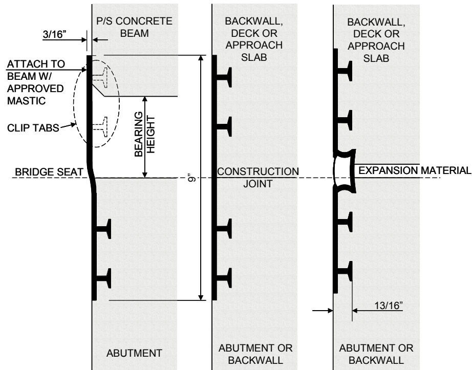
Figure 5.4.2 -1 Waterstop detail.
