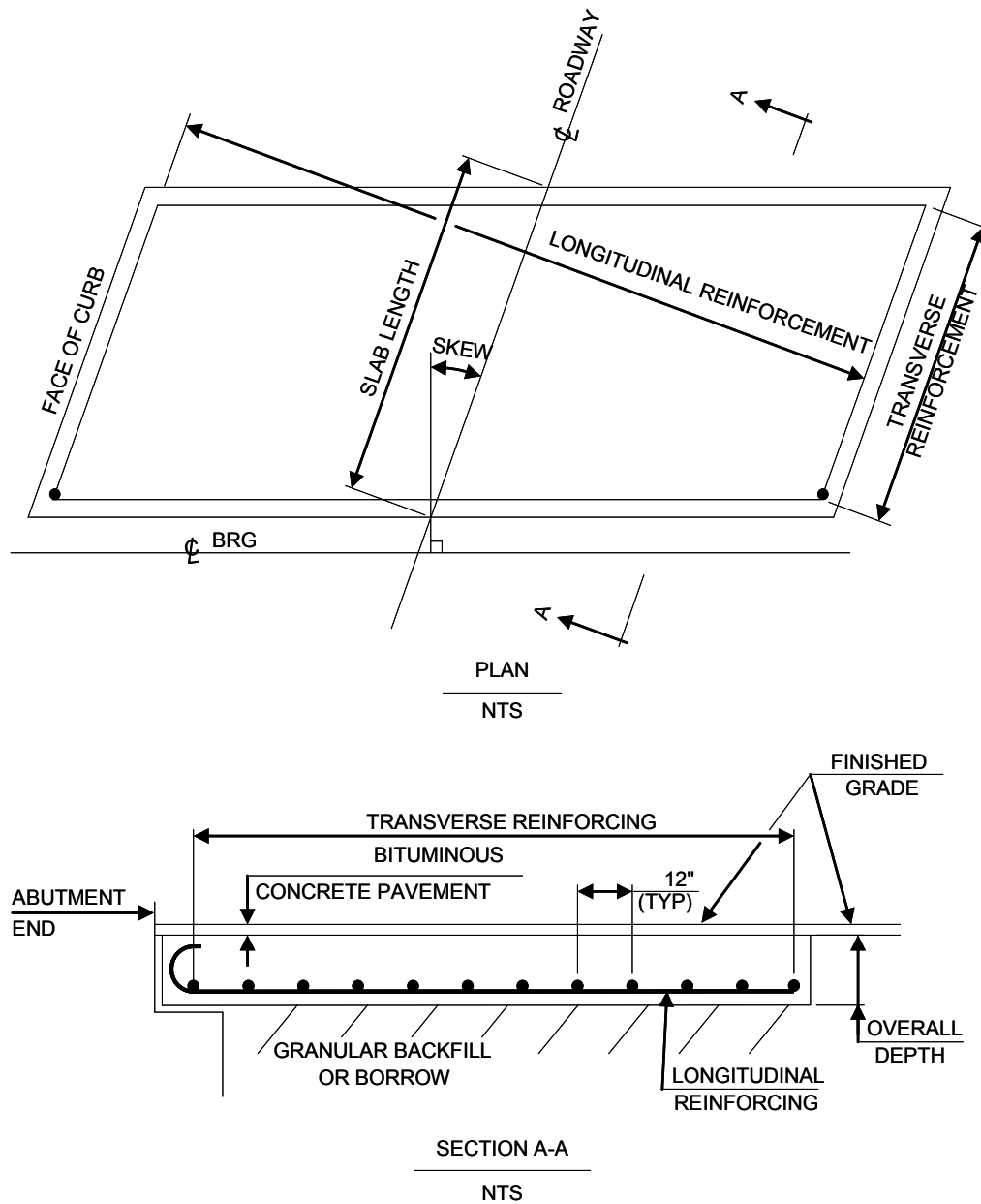
Figure 2.6.2 -1 Approach Slab Detail
