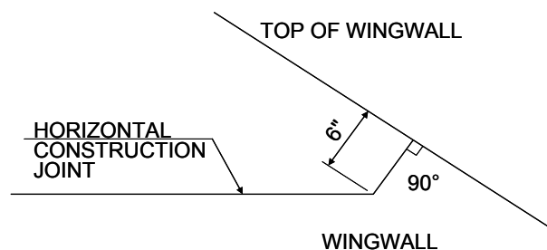
Figure 5.2.2.1 -1 Horizontal construction joint in wing wall.
