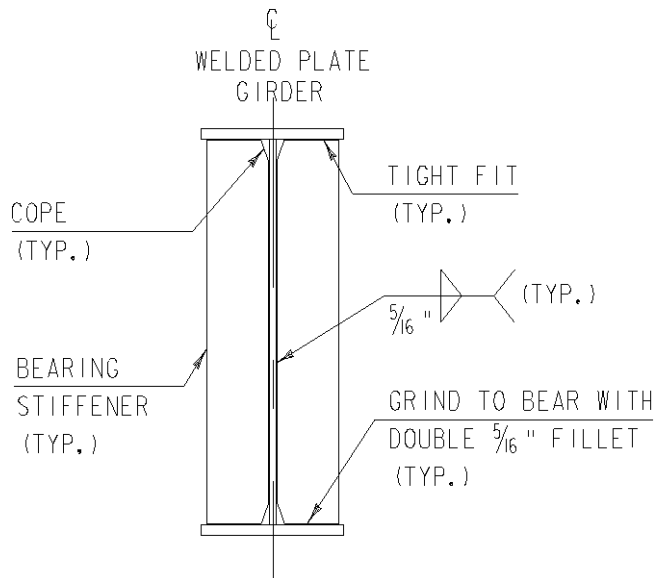
Figure 6.4.3 -4 Pier bearing stiffeners for welded plate girders
