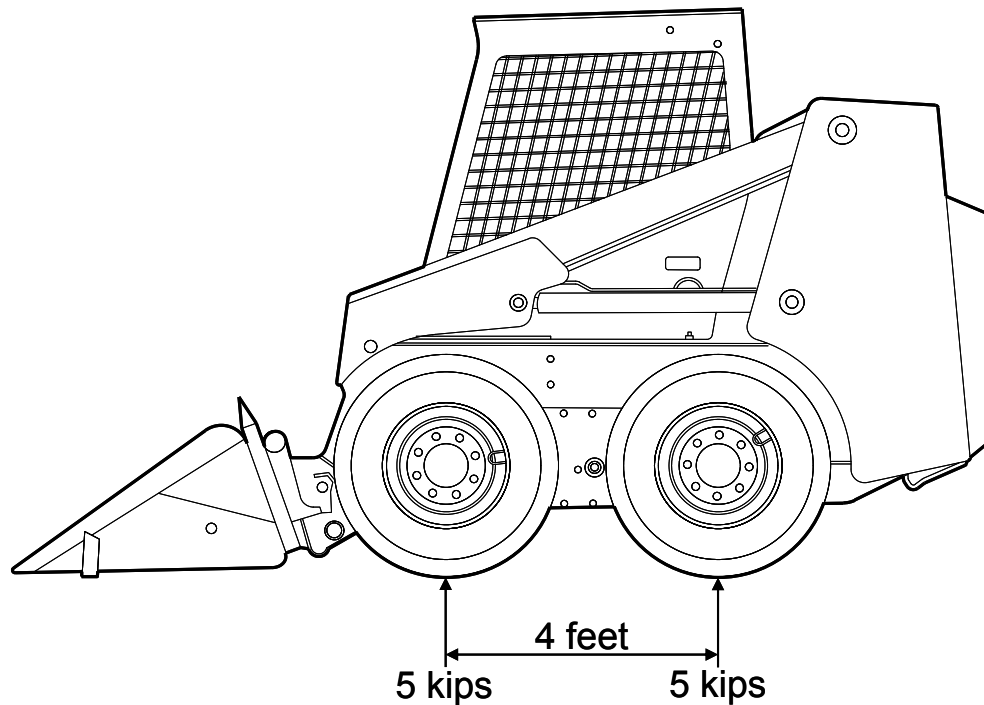
Figure 3.4.6 -1 Skid Steer Snow Removal Vehicle
