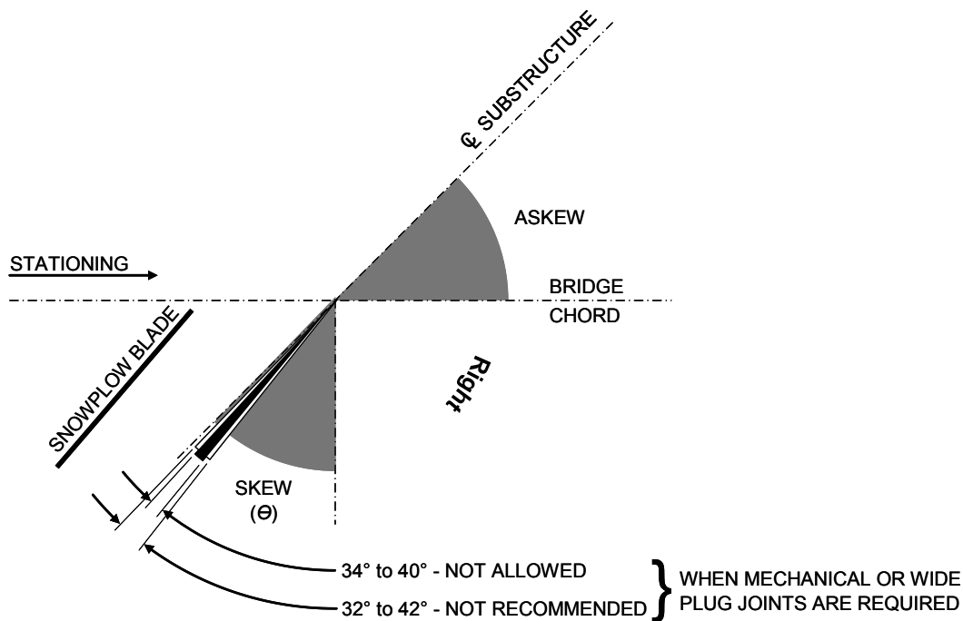
Figure 2.3.2-1 Skew and Askew Definition
