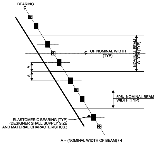
Figure 14.3.2-1 Layout of bearings for all spans.
