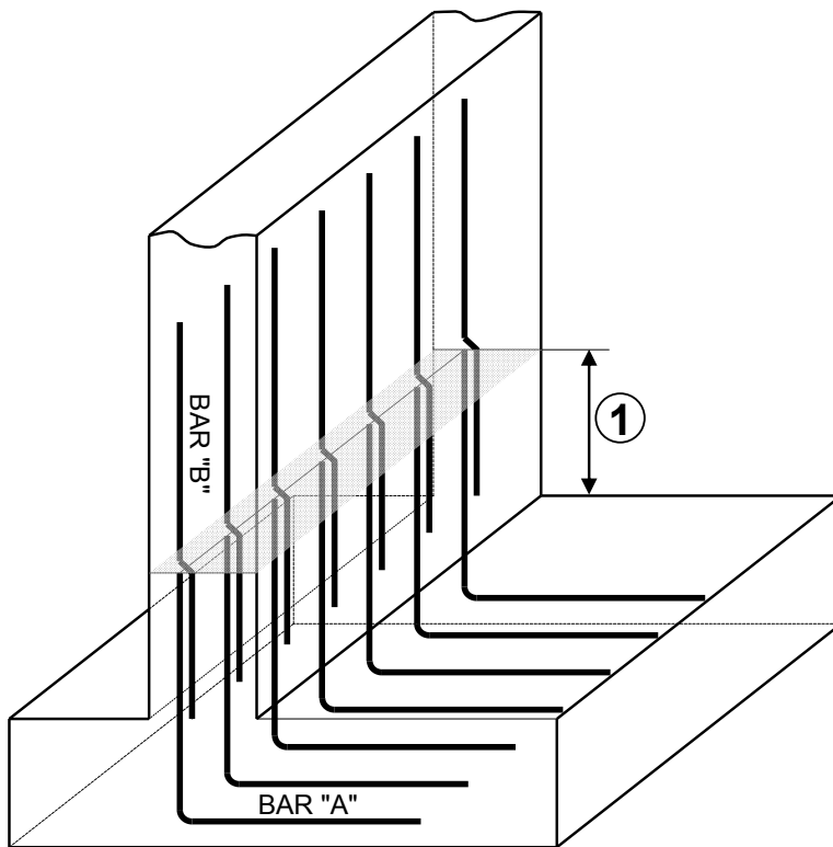
Figure 5.5.5 -2 Cat. 2: Bars Spliced at the Footing
