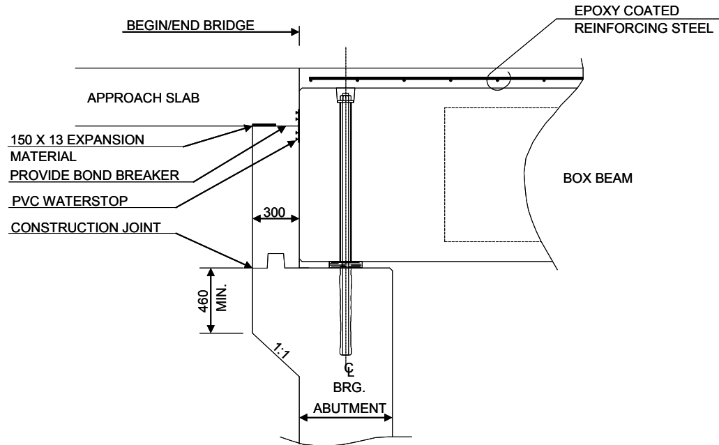
Figure 5.7.7-1 Box Beam Type G Bridge End Detail
