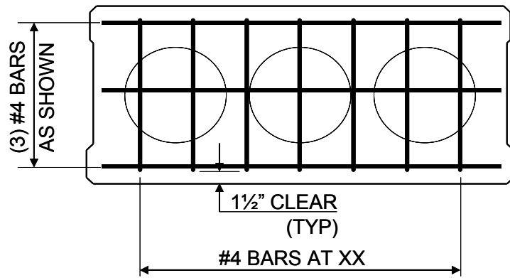
SECTION B – B END REINFORCING SECTION
