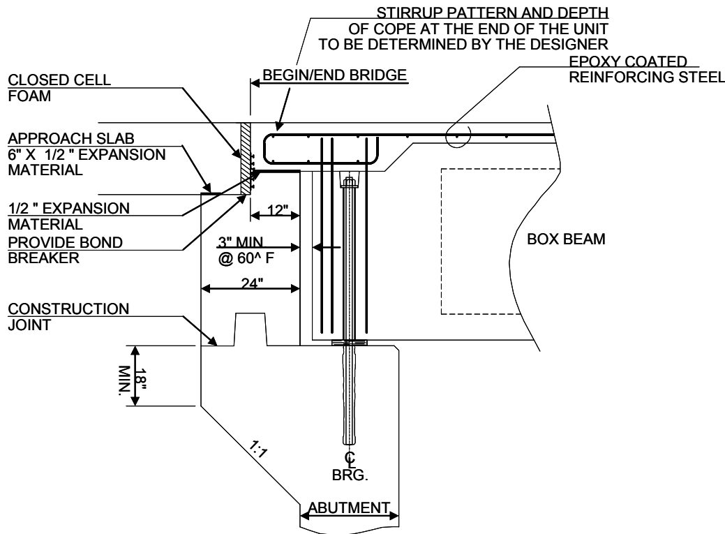
Figure 5.7.8 -1 Box Beam Type H Bridge End Detail
