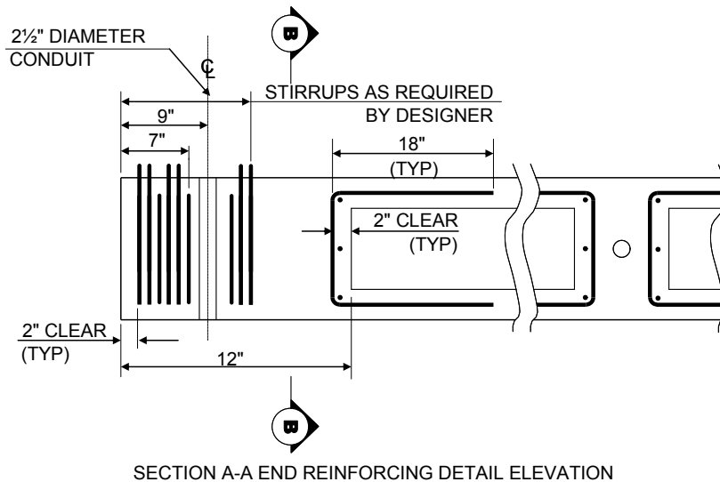
SECTION A-A END REINFORCING DETAIL ELEVATION
