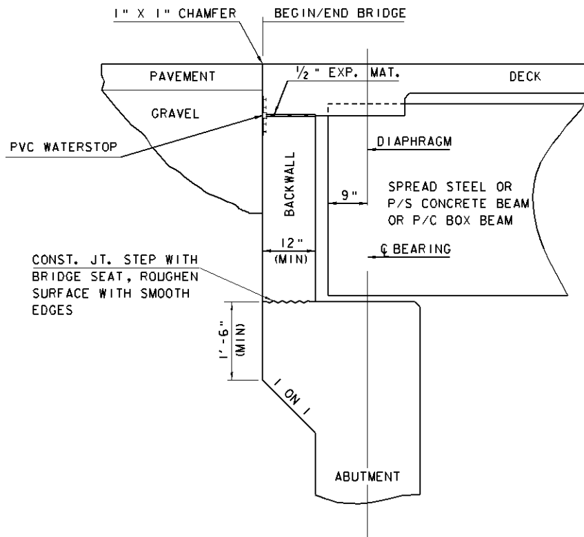
Figure 2.5.2.9 -1 Type I – Expansion and Fixed Bridge Ends for Long Span Spread Beam Decking without Approach Slabs of any skew or for the Expansion End of Butted Box Beam Decks with skews greater than 30°.
