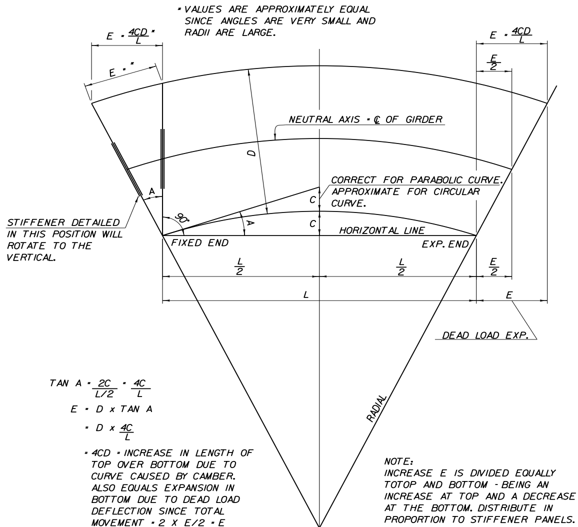
Figure 6.3.1.1 -1 Welded girders principles of girder camber calculations
