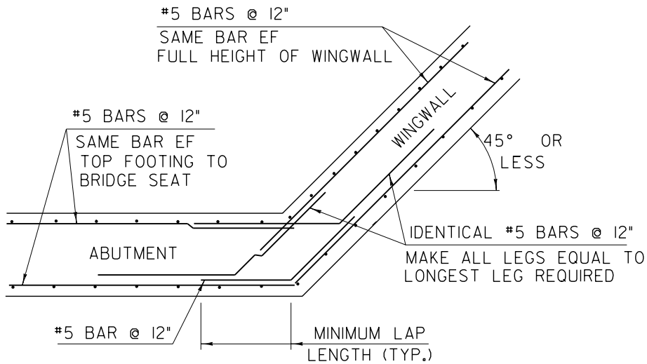
Figure 5.2.7.2 -1 Wing wall corner detail for 45° or under
