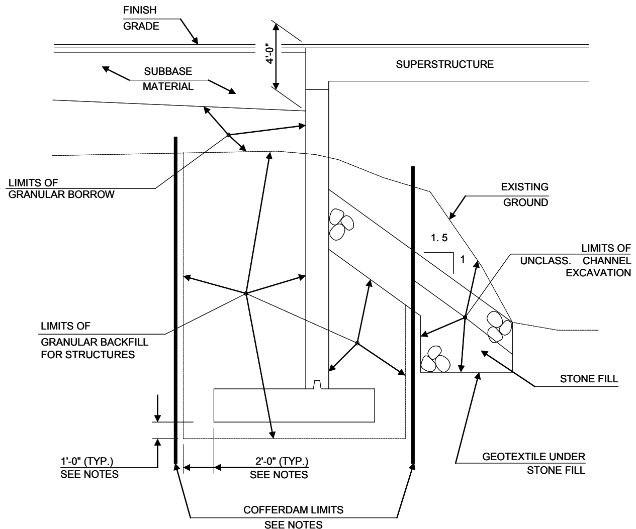
Figure 2.8.1.1-1 Typical Abutment Section Showing Cofferdam
