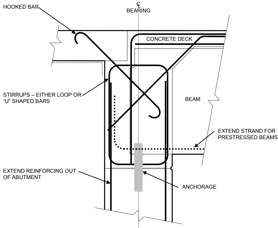
Figure 5.4.3 -1 Negative Moment Reinforcement.
