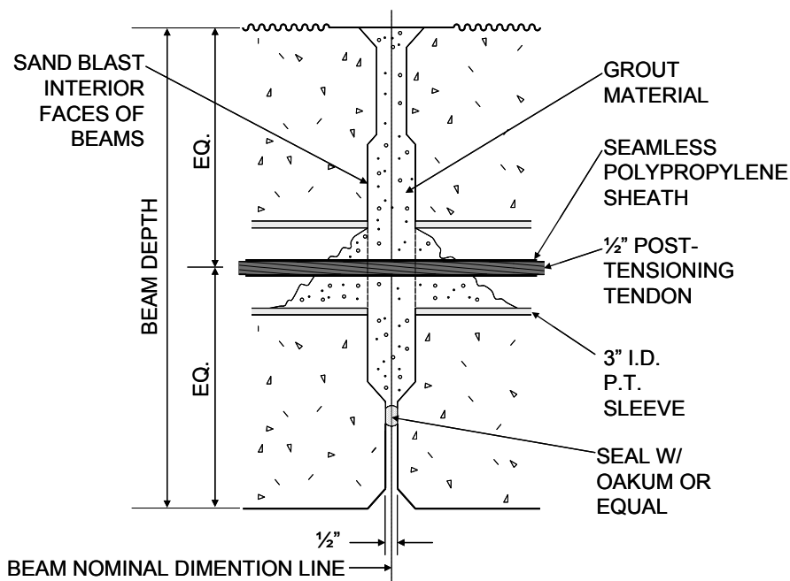
Figure 5.3.6 -1 Longitudinal joint section at transverse tendon.
