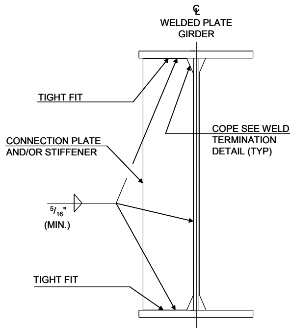
Figure 6.4.3 -5 Intermediate connection plates and/or stiffeners for welded plate girders
