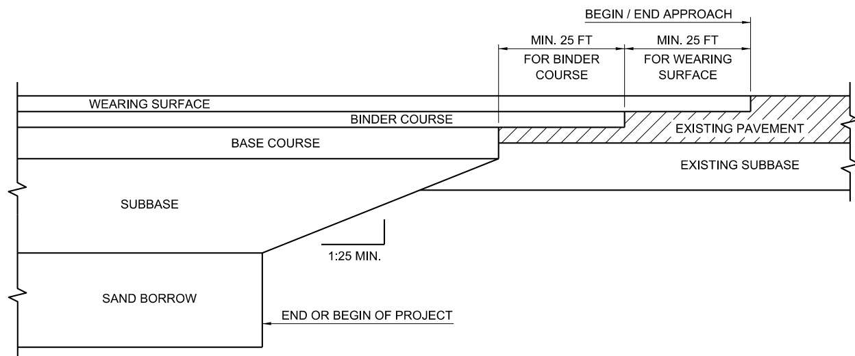
Figure 2.1.4 -1 Approach Detail
