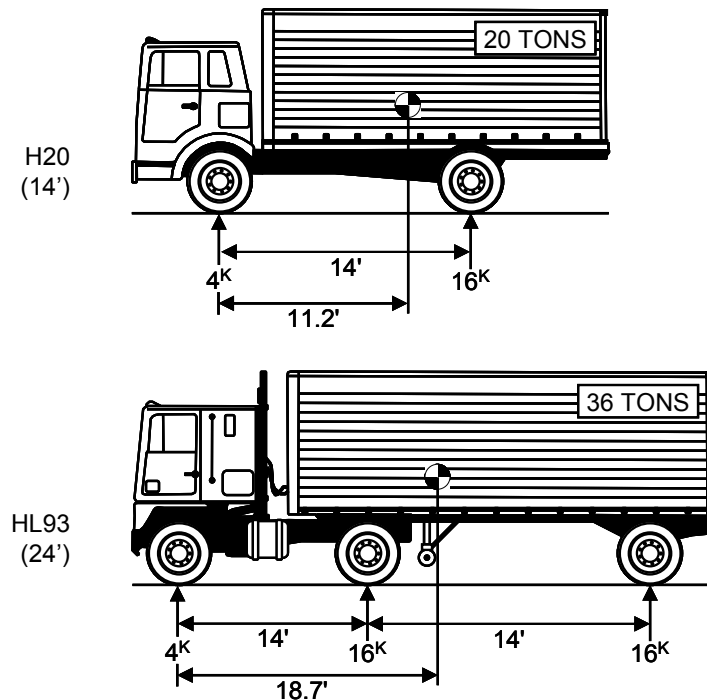
Figure 15.2.1-1 The AASHTO Standard Trucks
