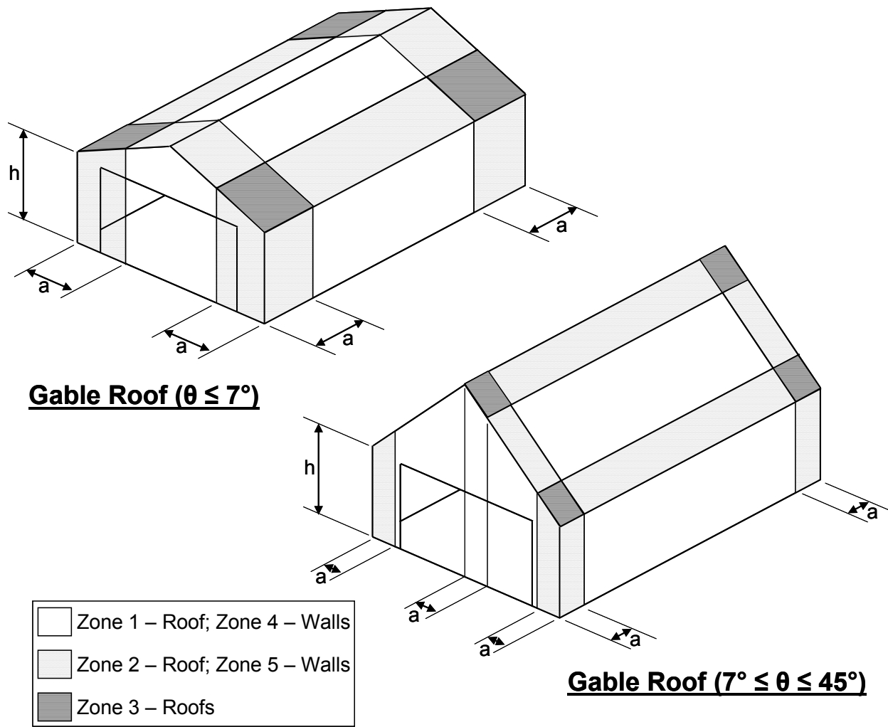
Figure 3.6.3.6.2 -1 Components and Cladding Pressure (Source: ASCE 7-05 Figure 6-3)
