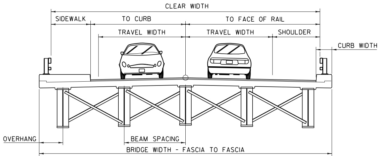
Figure 2.1.3 -1 Bridge Typical
