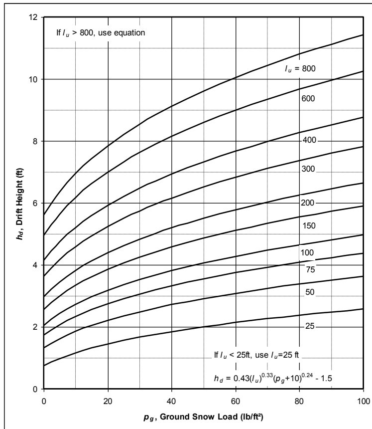
Figure 3.7.2.2.2 -2 Graph and Equation for Determining Drift Height, h_d
