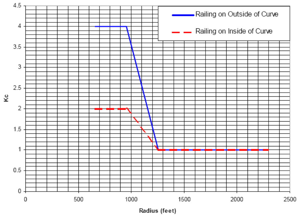
Figure 13.4-2 Curvature Traffic Adjustment Factor (Kc)
