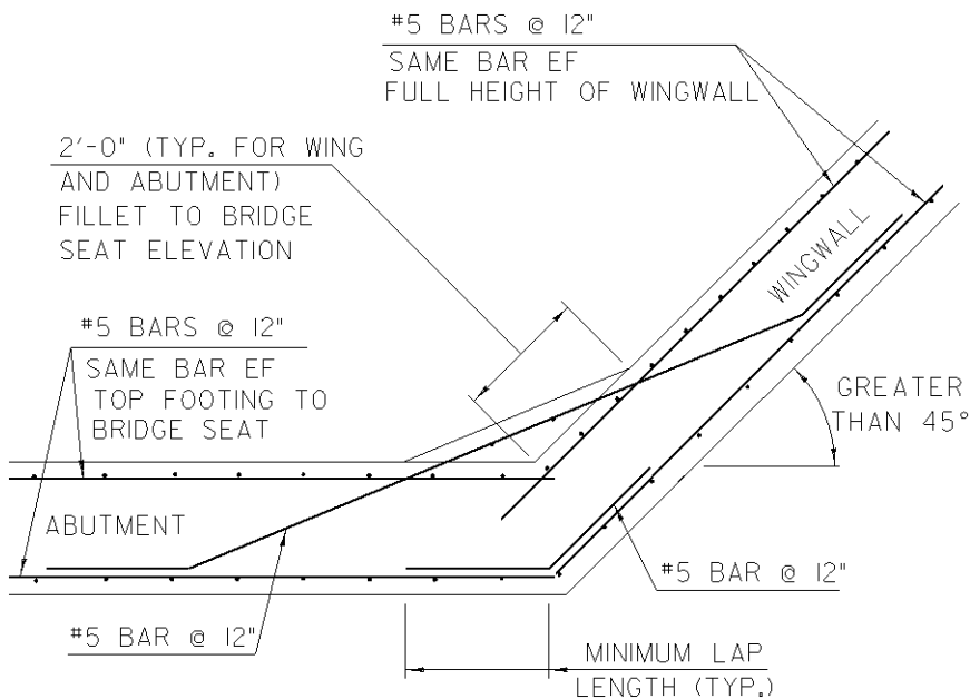
Figure 5.2.7.2 -2 Wing wall corner detail for more than 45° angle
