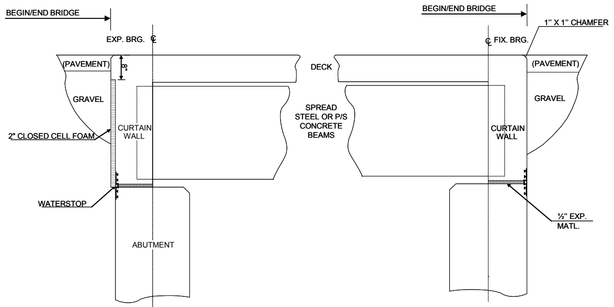
Figure 2.5.2.5 -1 Type E – Bridge Ends for intermediate spans without Approach Slabs.
