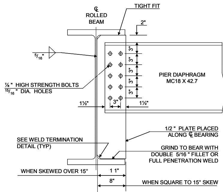
Figure 6.3.3.3.1-1 Pier diaphragms for continuous rolled beam bridges
