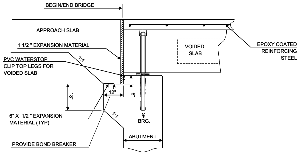
Figure 5.7.3 -2 Voided Slab Type C Bridge End Detail
