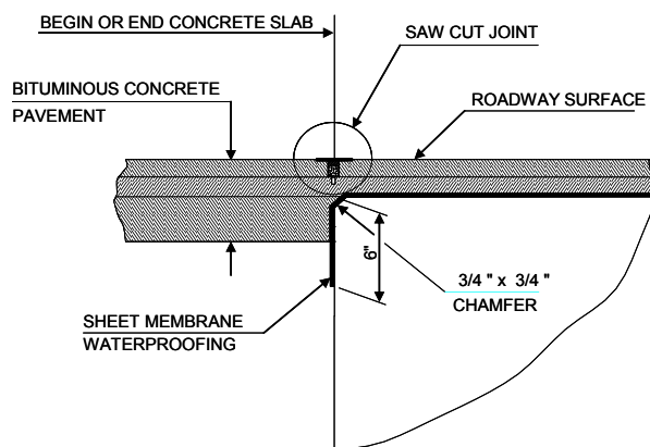
Figure 14.2.1.4 -1 Saw Cut Joint Detail
