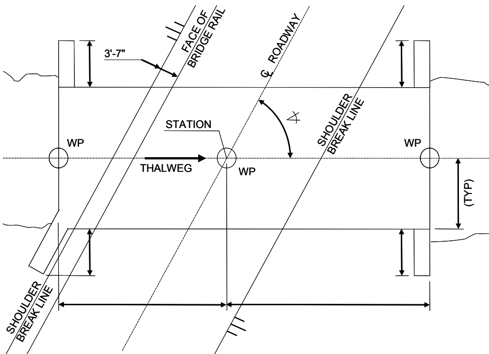
Figure 2.3.1-3 Pipe, Small Box or Small Frame
