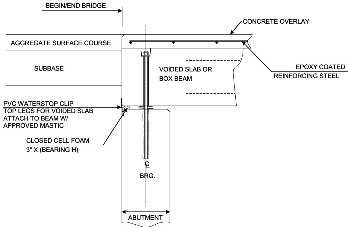
Figure 5.7.4 -2 Voided Slab and Box Beam Type D Bridge End Detail
