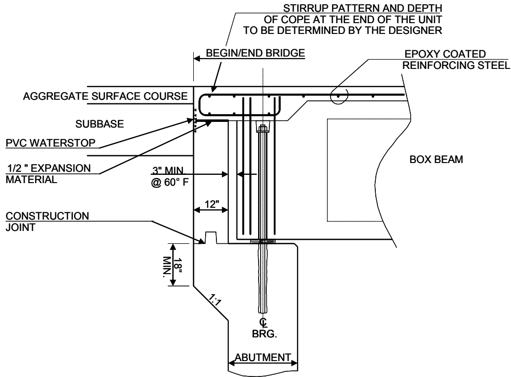
Figure 5.7.9 -1 Box Beam Type I Bridge End Detail
