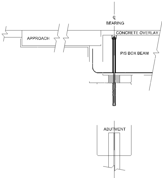
Figure 5.7.1 -1 Box Beam Type A Bridge End Detail
