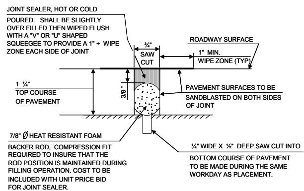
Figure 14.2.1.4 -2 Saw Cut Joint Detail Close Up
