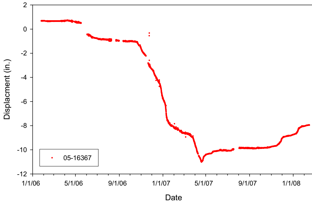
Figure 5.24 Calculated displacement for IPI 05-16367 installed at a depth of 6.86m (22.5 ft.) in Inclinator #2.
