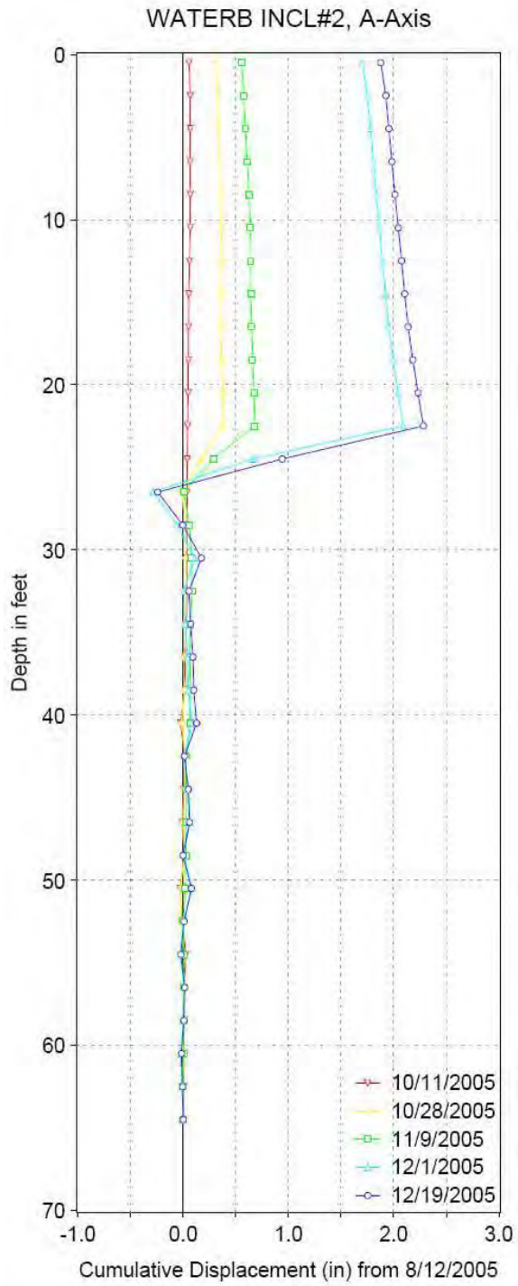
Figure B.2 Inclinometer #2 cumulative displacement profiles.
