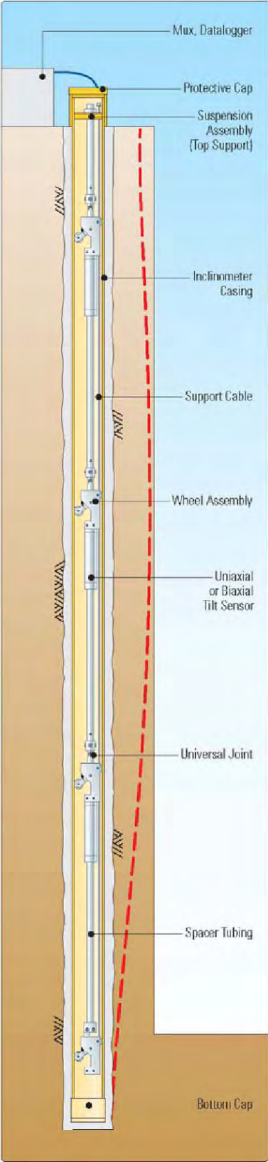
Figure 2.2 Typical IPI installation including three inclinometers (Geokon 2007).
