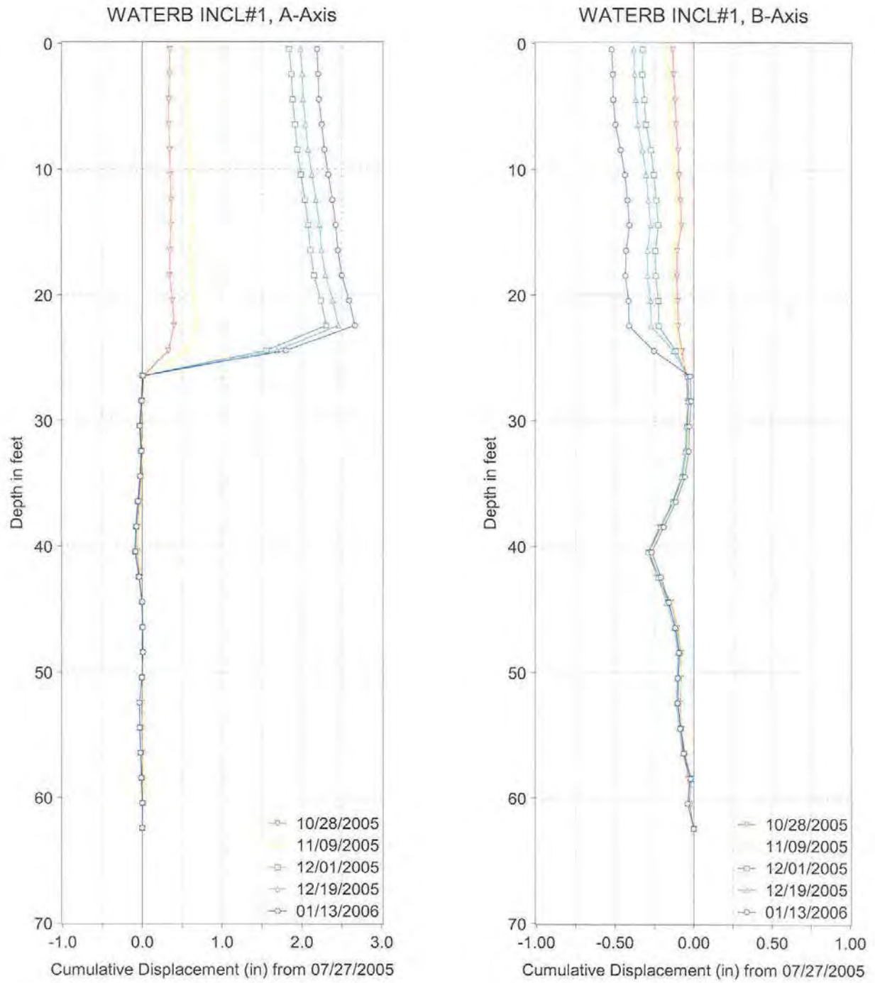
Figure B.1 Inclinerometer #1 cumulative displacement profiles.
