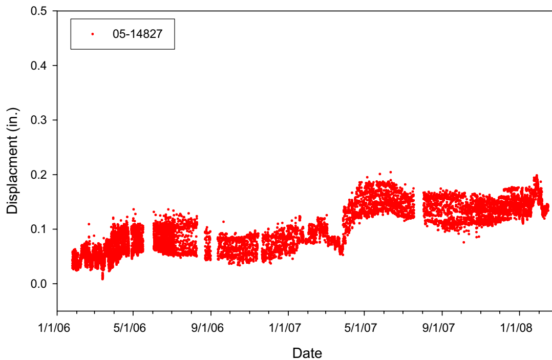
Figure 5.16 Calculated displacement for IPI 05-14827 installed at a depth of 3.81m (12.5 ft.) in Inclinator #3.
