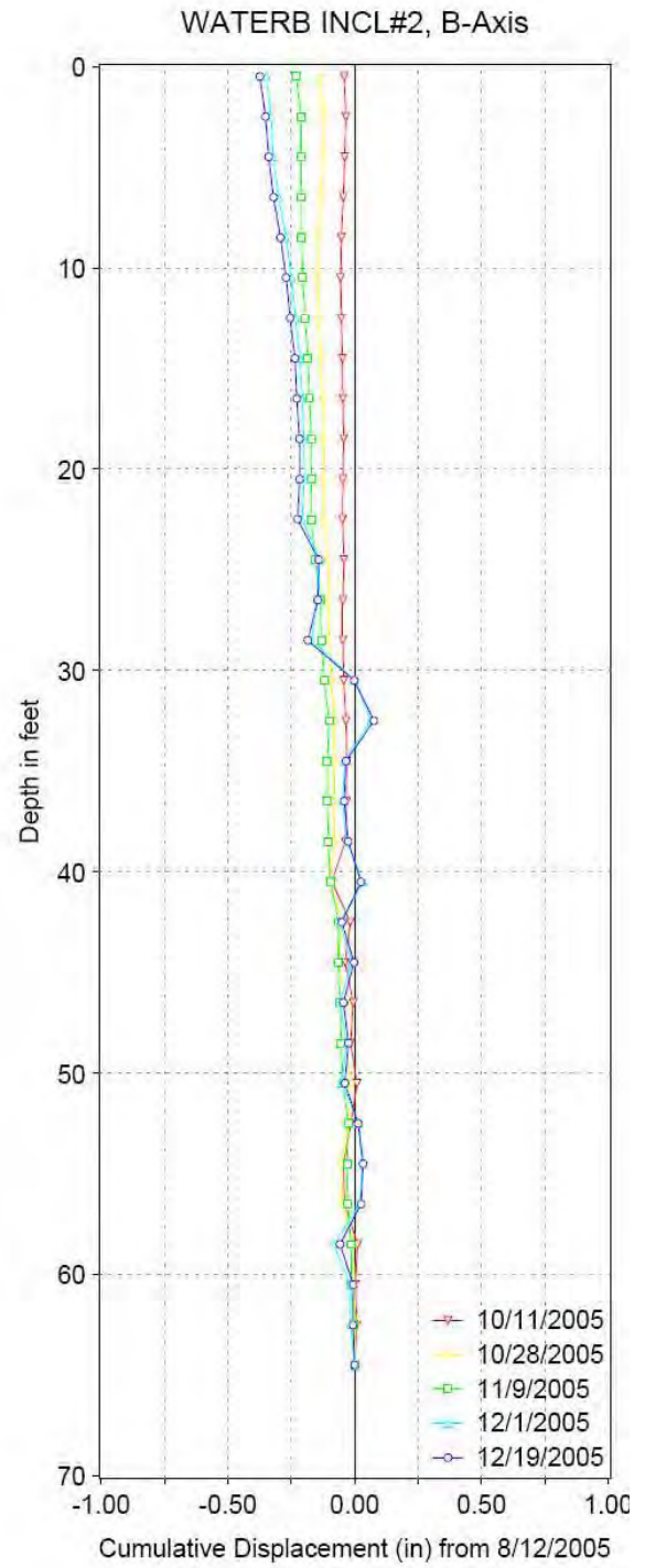
Figure B.2 Inclinometer #2 cumulative displacement profiles.
