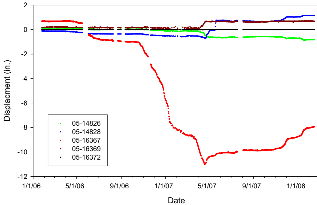
Figure 5.20 Calculated displacements for each IPI installed in Inclinator #2.
