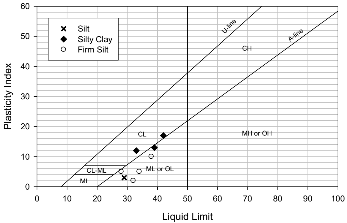
Figure 4.6 Casagrande's plasticity chart for Inclinator 1.
