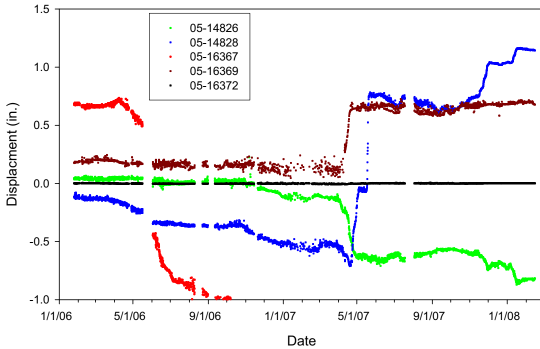
Figure 5.21 Calculated displacements for each IPI installed in Inclinator #2 when the displacement scale has been reduced.
