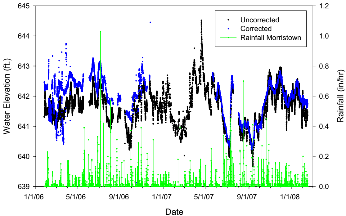
Figure 5.8 Corrected and uncorrected water table elevations for Monitoring Well #1 compared to measured rainfall at Morrystown Airport.
