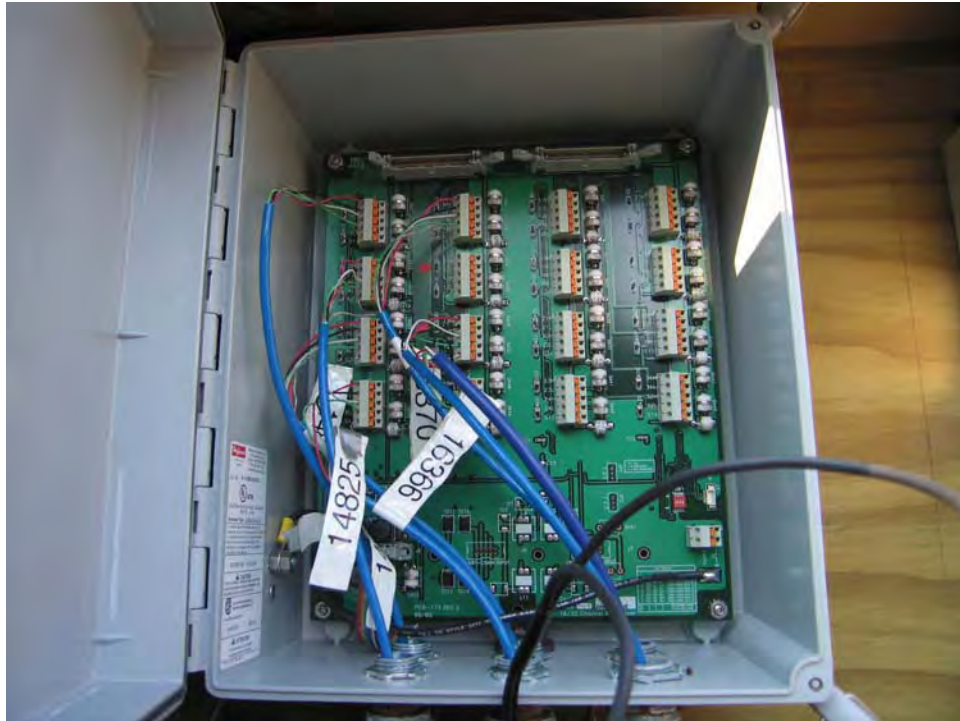
Figure 3.11 Geokon 8032 multiplexer.
