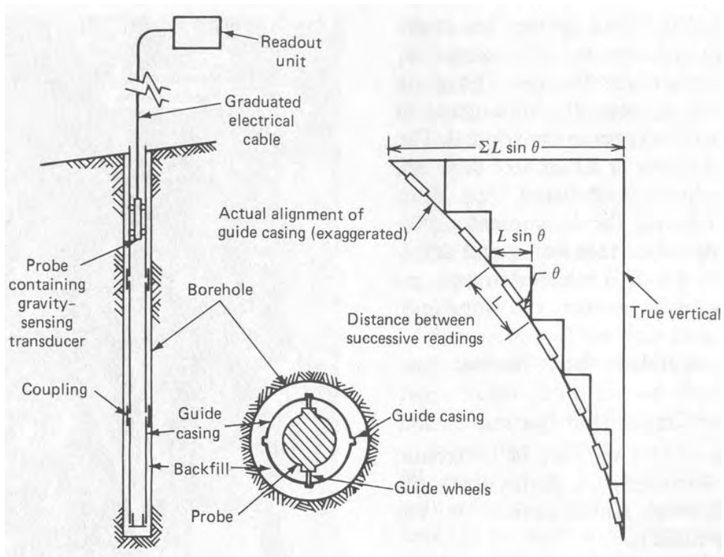
Figure 5.12 Principal of inclinometer operation (Dunncliff, 1988)
