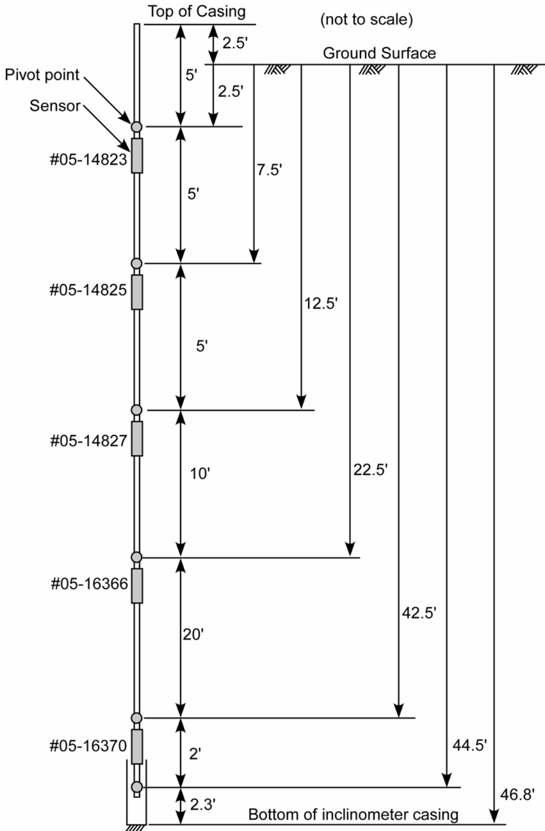
Figure 3.5 Sketch of installed IPIs in Inclinometer #3.
