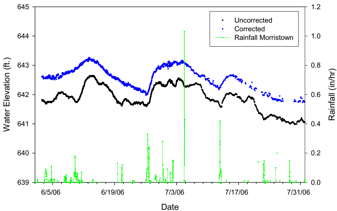
Figure 5.9 Corrected and uncorrected water table elevations for Monitoring Well #1 compared to measured rainfall at Morrystown Airport for June and July, 2006.
