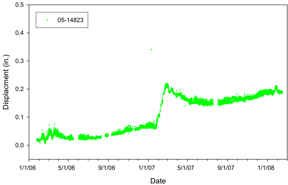
Figure 5.14 Calculated displacement for IPI 05-14823 installed at a depth of 0.76m (2.5 ft.) in Inclinometer #3.
