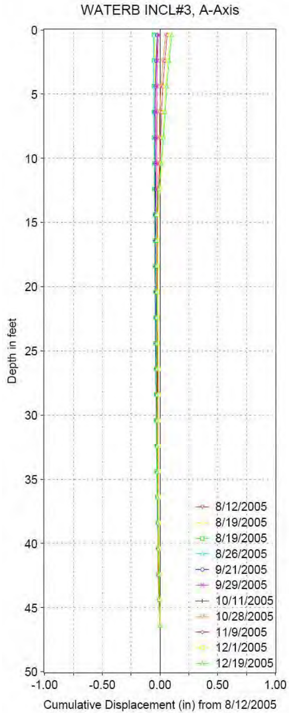
Figure B.3 Inclinerometer #3 cumulative displacement profiles.
