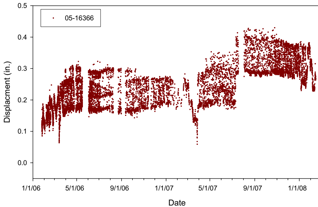
Figure 5.17 Calculated displacement for IPI 05-16366 installed at a depth of 6.86m (22.5 ft.) in Inclinator #3.
