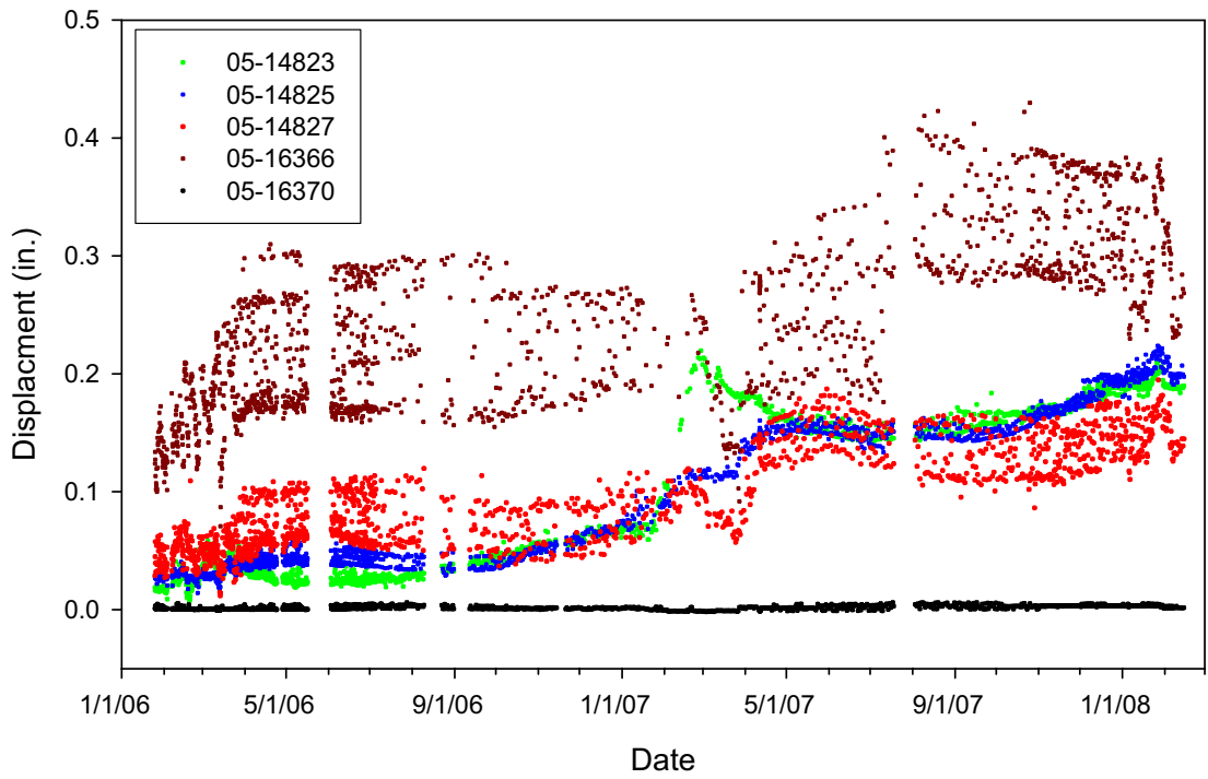
Figure 5.13 Calculated displacements for each IPI installed in Inclinometer #3.
