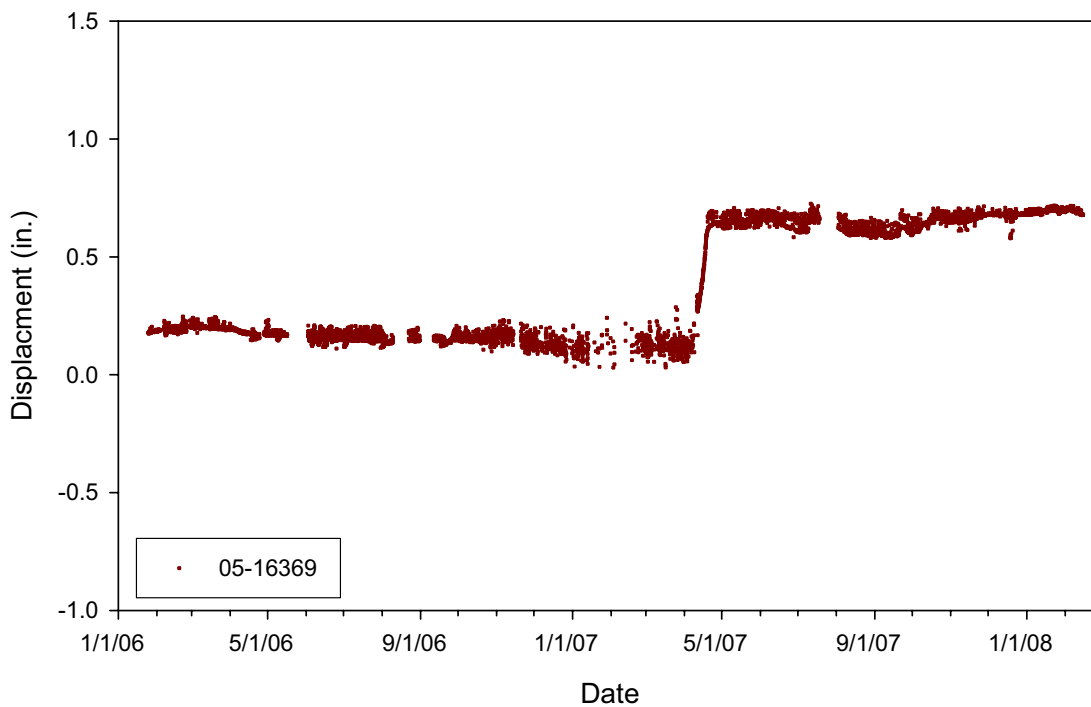
Figure 5.25 Calculated displacement for IPI 05-16369 installed at a depth of 12.95m (42.5 ft.) in Inclinator #2.
