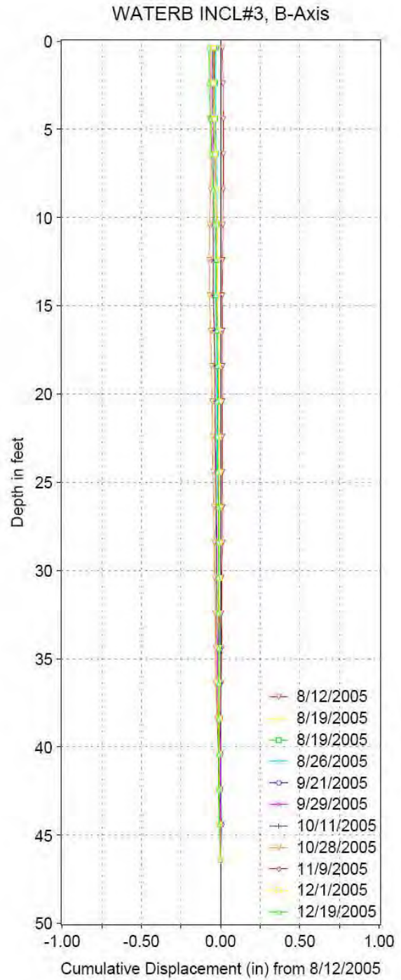
Figure B.3 Inclinerometer #3 cumulative displacement profiles.
